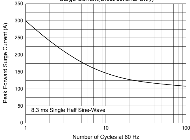
Fig. 5 - Maximum Non-Repetitive Peak Forward Surge Current(Unidirectional Only)
