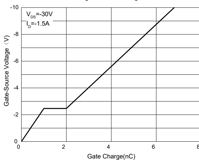
Fig. 6 - Gate Charge
