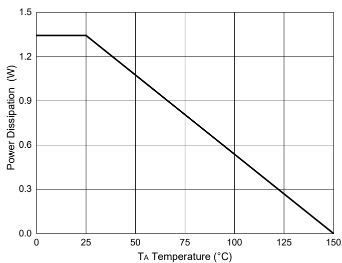
Fig.11-PD Dissipation
