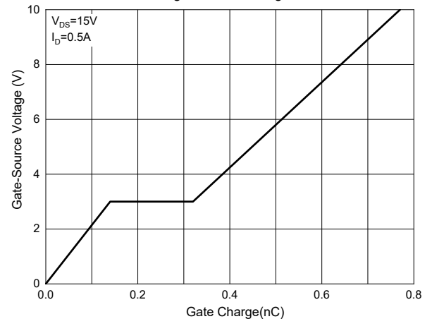
Fig. 6 - Gate Charge
