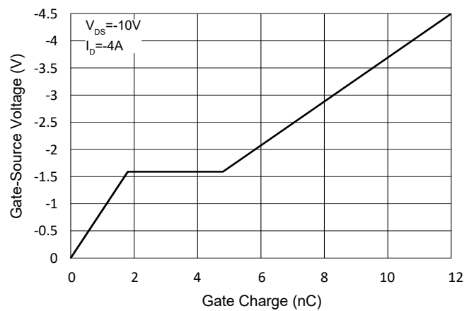
Fig.6 - Gate Charge
