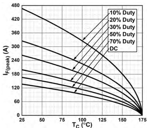
Fig. 7 - Current Derating
