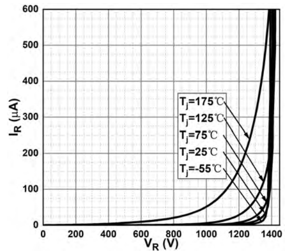
Figure 2. Reverse Characteristics
