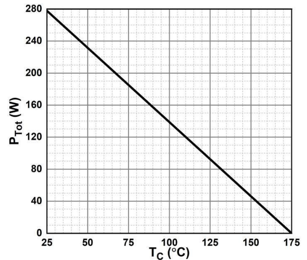
Figure 6. Power Derating
