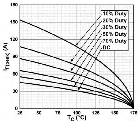
Fig. 7 - Current Derating
