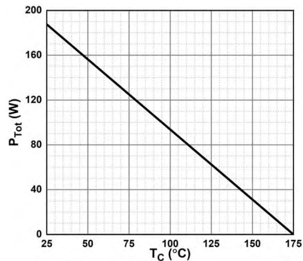
Figure 6. Power Derating
