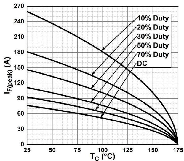
Fig. 7 - Current Derating
