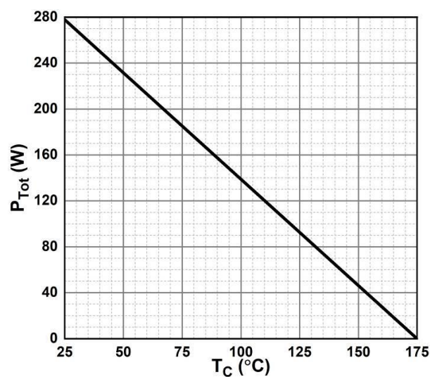
Figure 6. Power Derating
