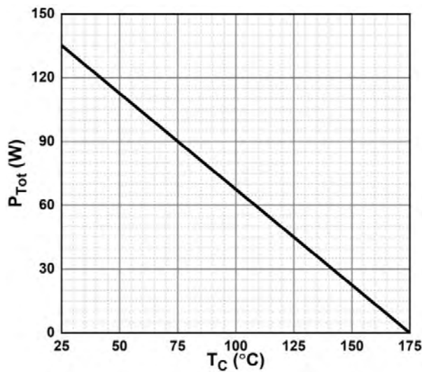
Figure 6. Power Derating
