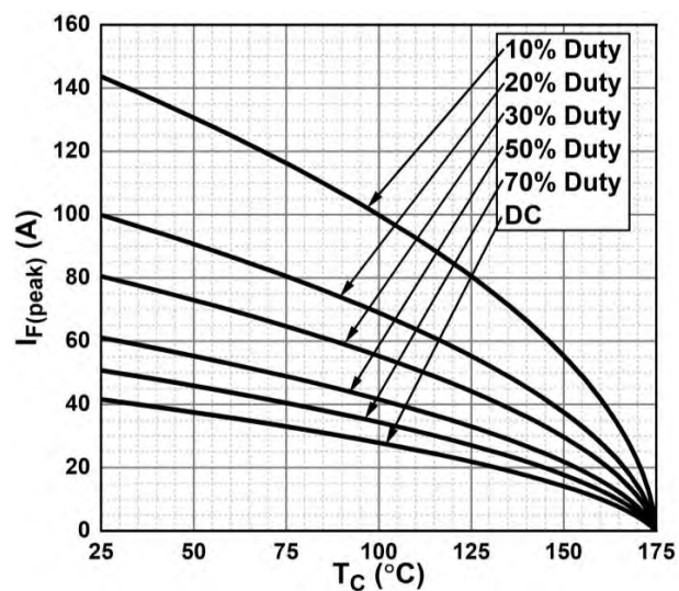
Fig. 7 - Current Derating
