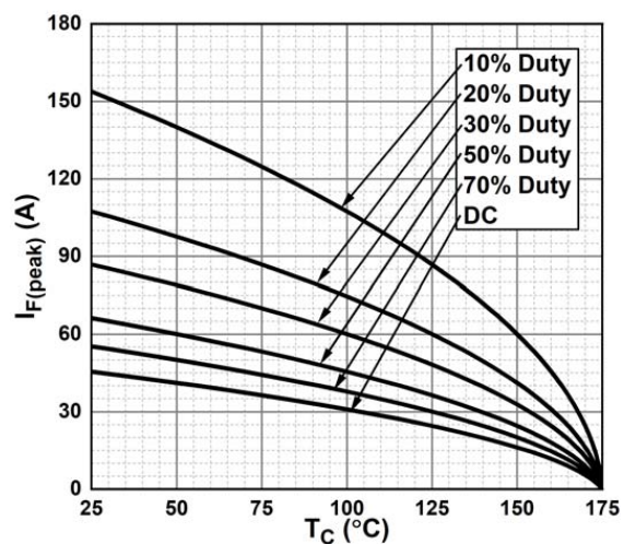
Fig. 7 - Current Derating
