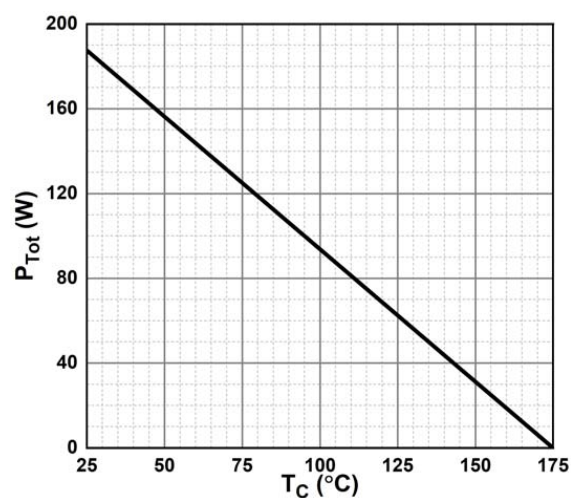
Figure 6. Power Derating
