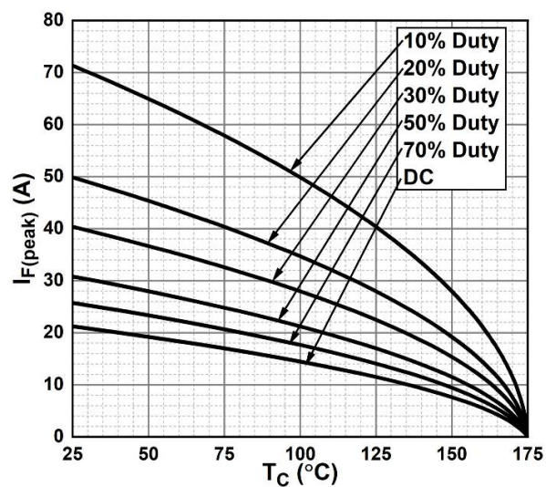
Fig. 7 - Current Derating
