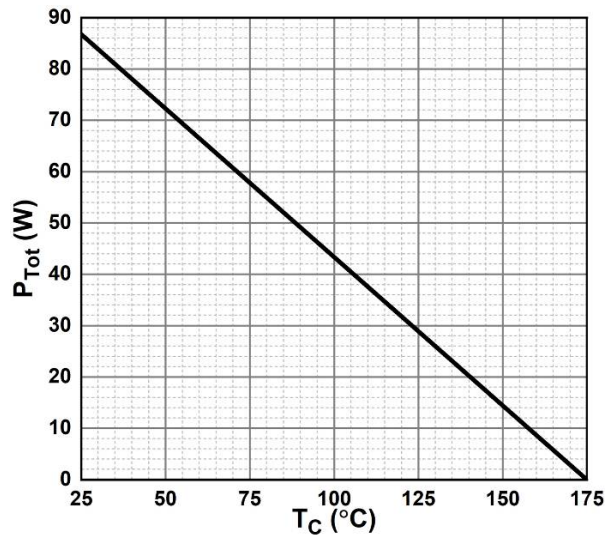
Figure 6. Power Derating
