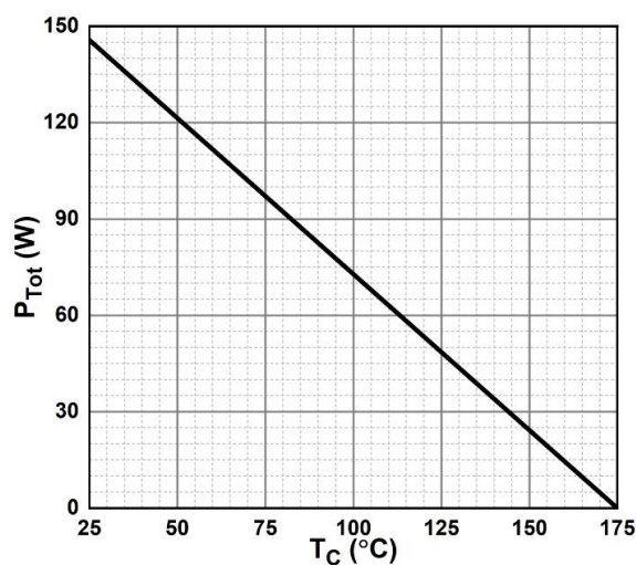
Figure 6. Power Derating
