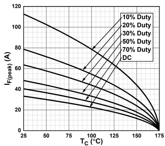
Fig. 7 - Current Derating
