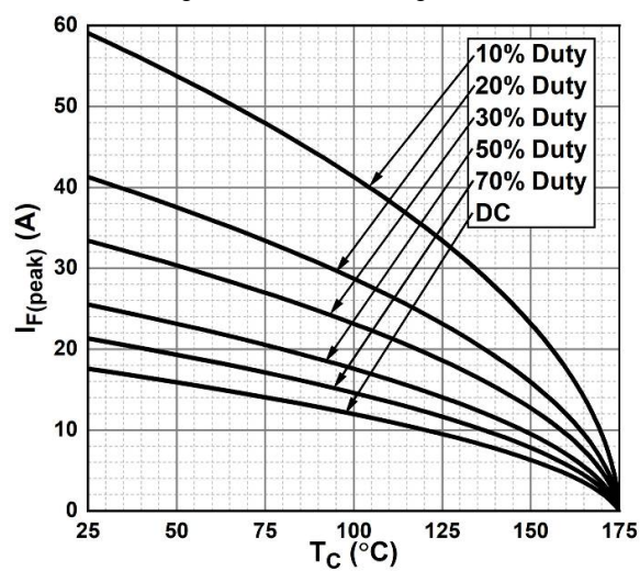
Fig. 7 - Current Derating
