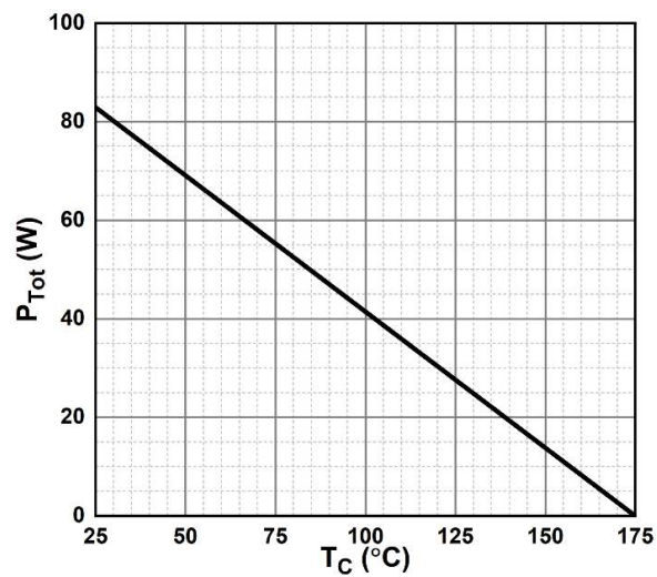
Figure 6. Power Derating
