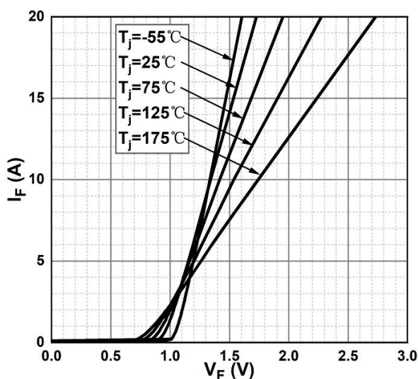
Figure 1. Forward Characteristics
