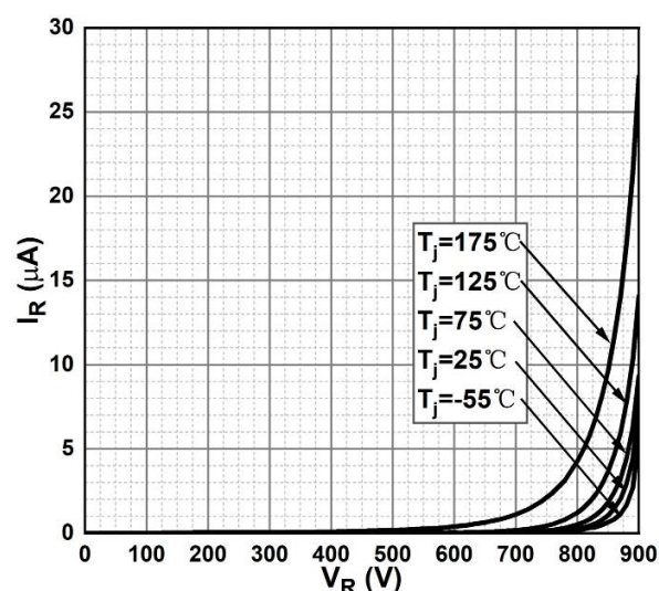
Figure 2. Reverse Characteristics
