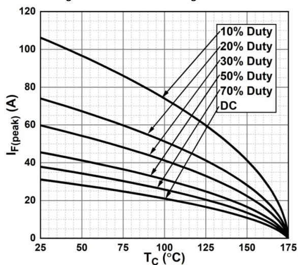
Figure 7. Current Derating
