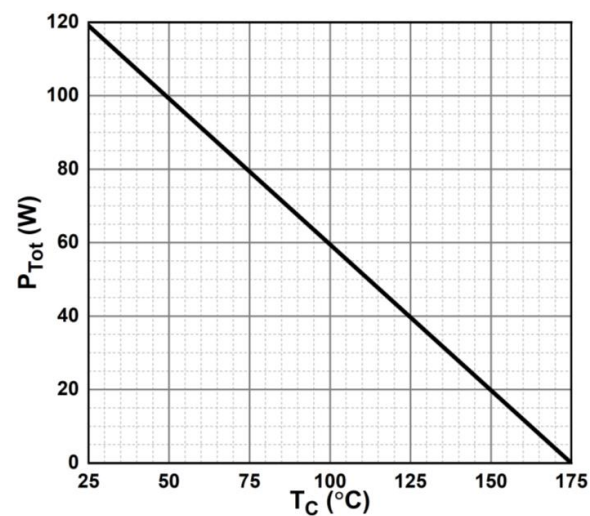
Figure 6. Power Derating
