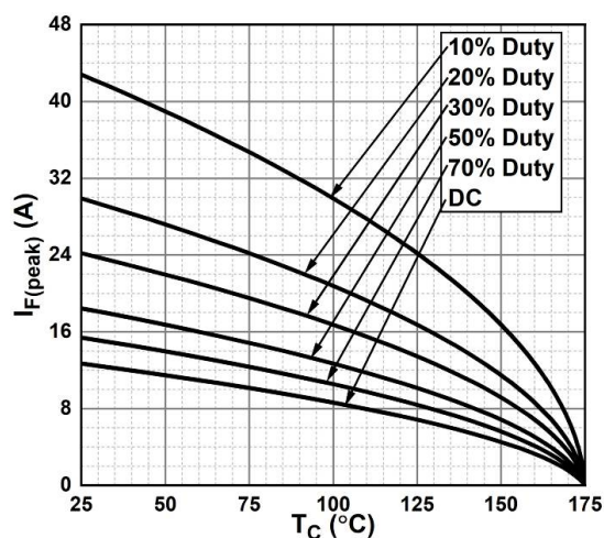
Figure 7. Current Derating
