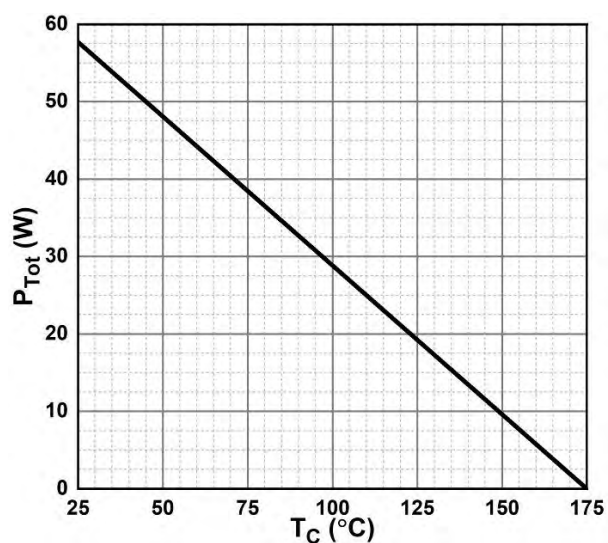
Figure 6. Power Derating
