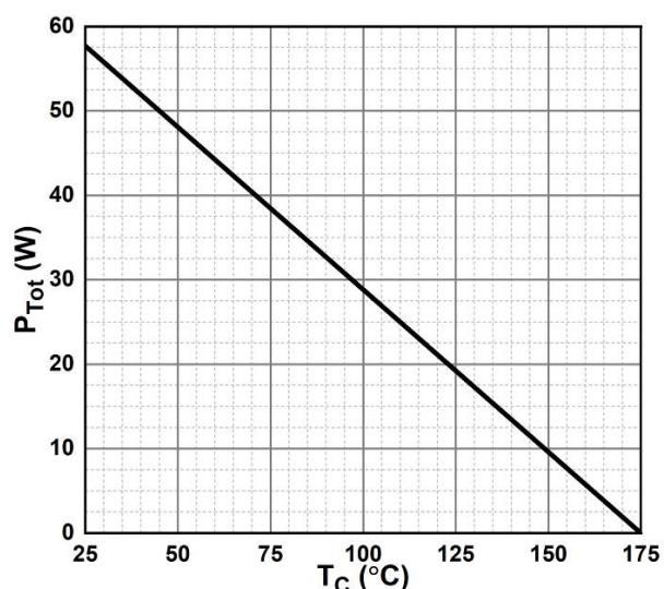
Figure 6. Power Derating
