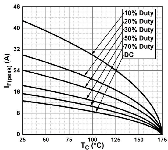
Figure 7. Current Derating
