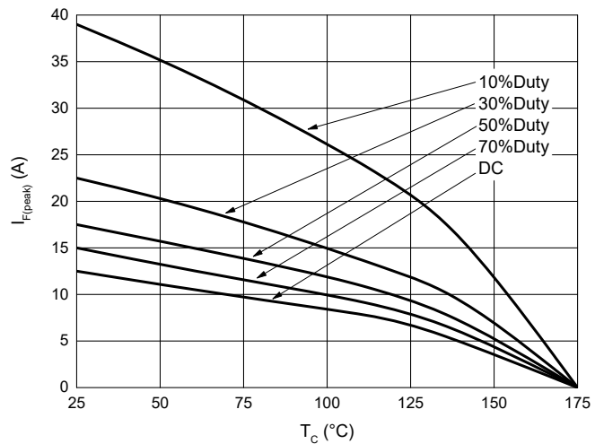
Fig. 7 - Current Derating
