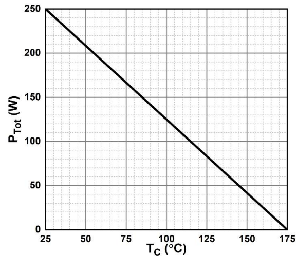
Figure 6. Power Derating
