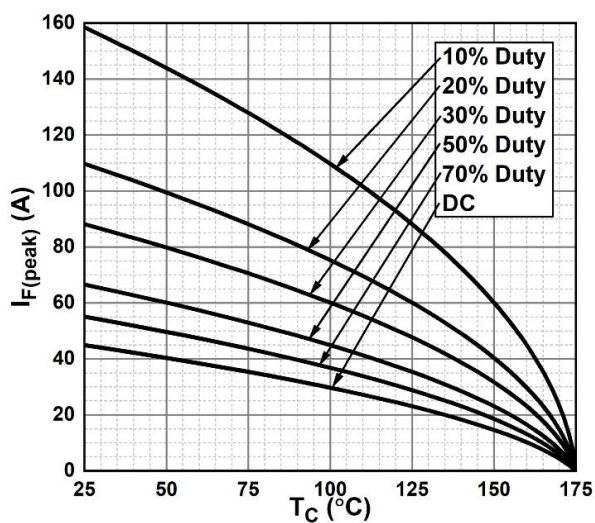
Figure 7. Current Derating
