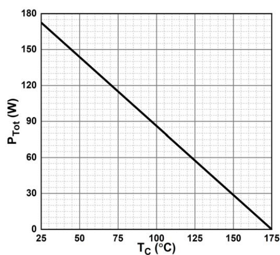
Figure 6. Power Derating
