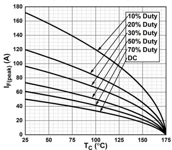
Figure 7. Current Derating
