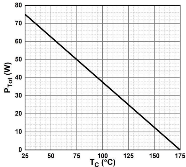
Figure 6. Power Derating
