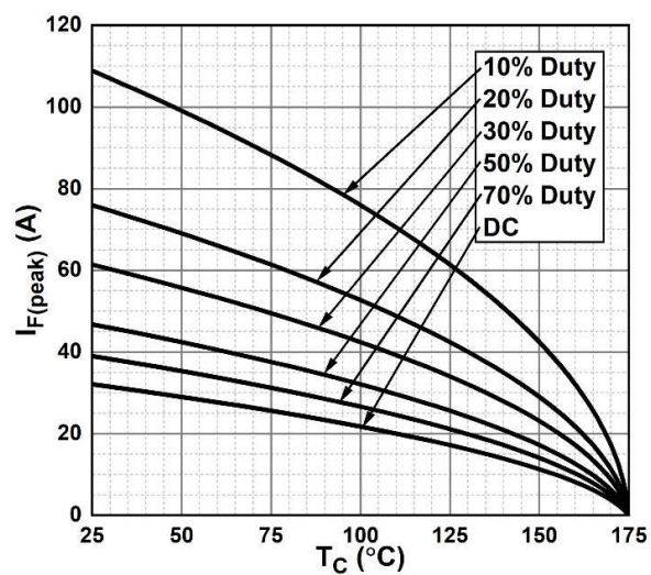
Figure 7. Current Derating
