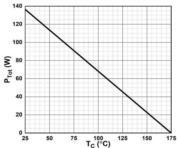
Figure 6. Power Derating
