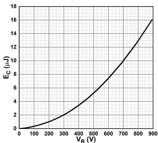
Figure 5. Capacitance Stored Energy
