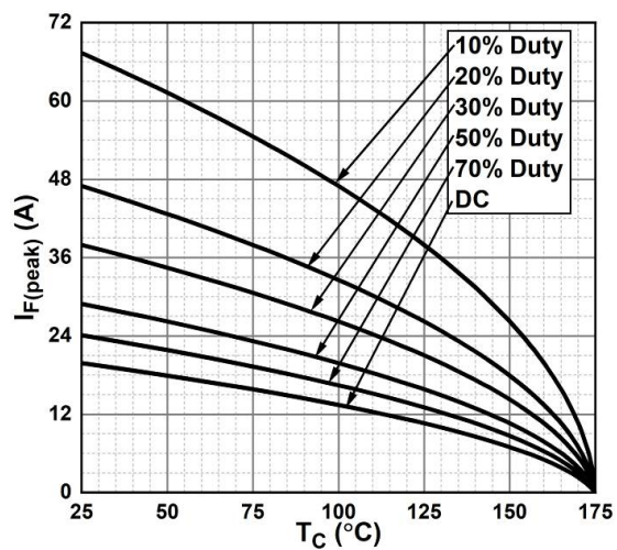
Figure 7. Current Derating
