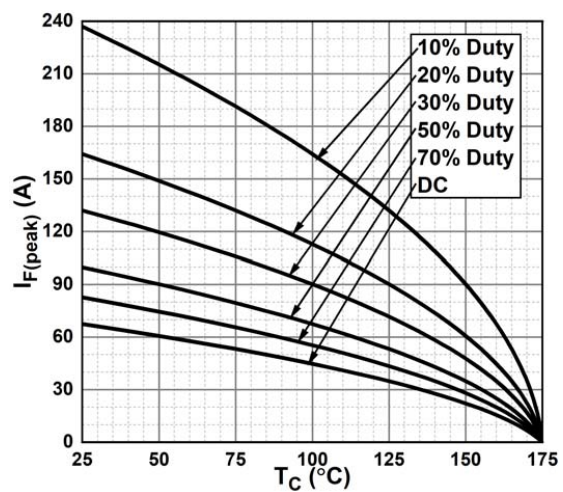
Fig. 7 - Current Derating
