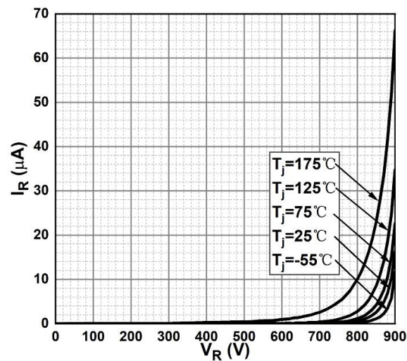
Figure 2. Reverse Characteristics
