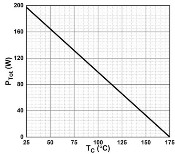
Figure 6. Power Derating
