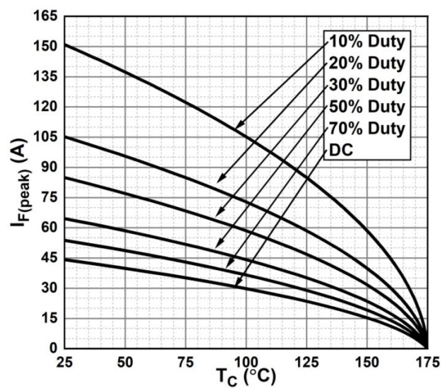
Fig. 7 - Current Derating
