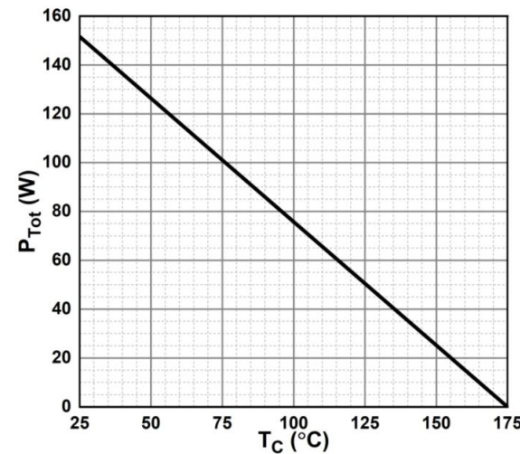
Figure 6. Power Derating
