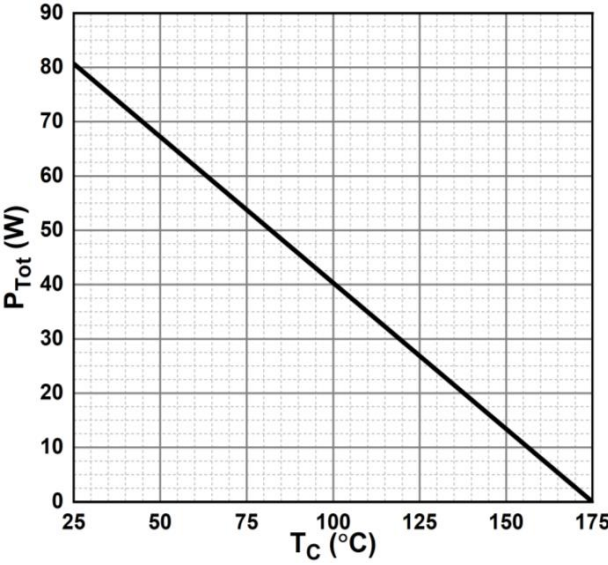
Figure 6. Power Derating
