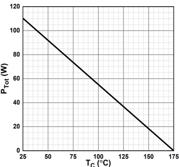
Figure 6. Power Derating
