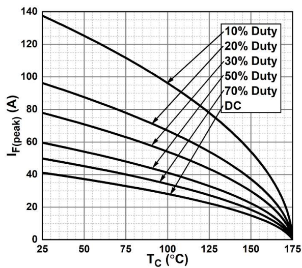
Fig. 7 - Current Derating
