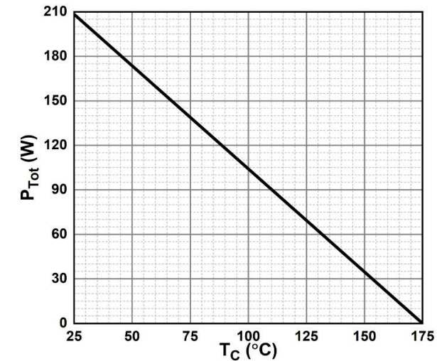
Figure 6. Power Derating
