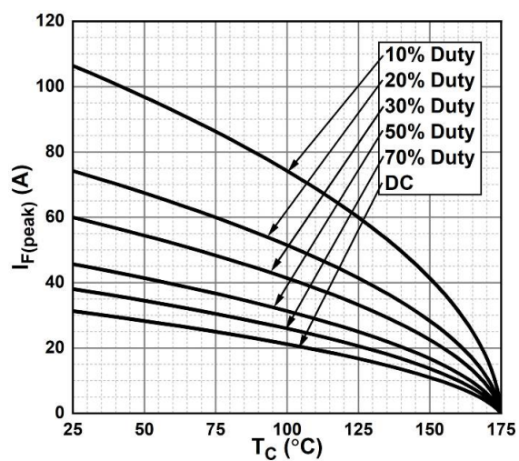
Fig. 7 - Current Derating
