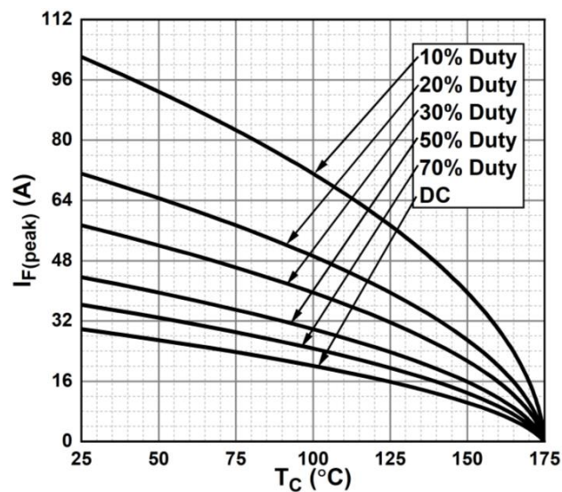
Fig. 7 - Current Derating
