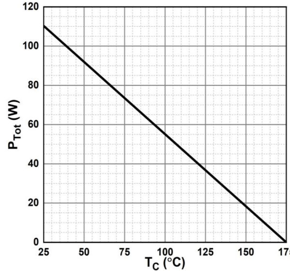
Figure 6. Power Derating
