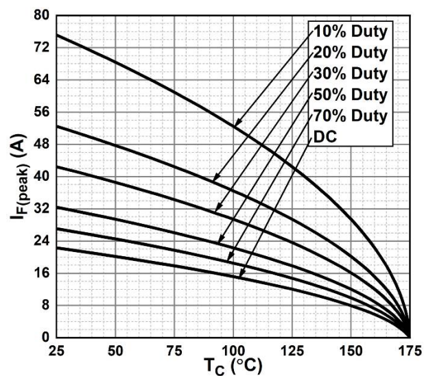
Fig. 7 - Current Derating
