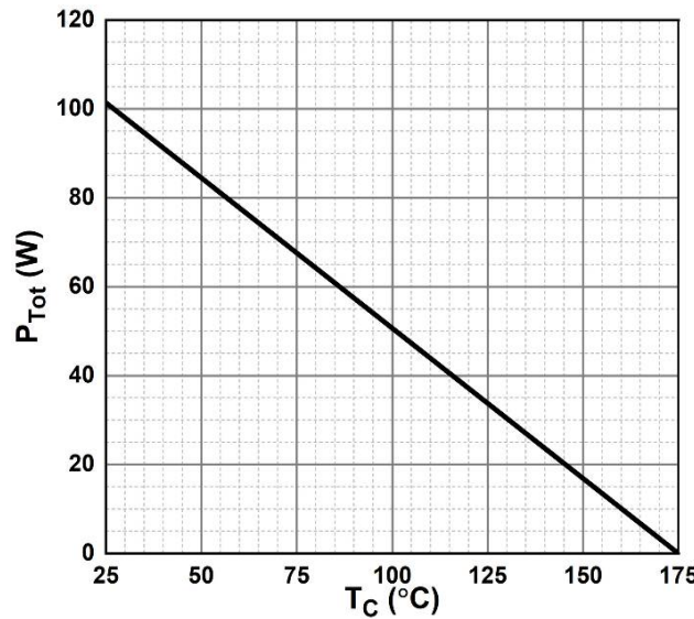
Figure 6. Power Derating
