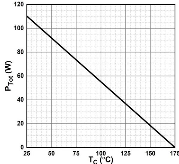
Figure 6. Power Derating
