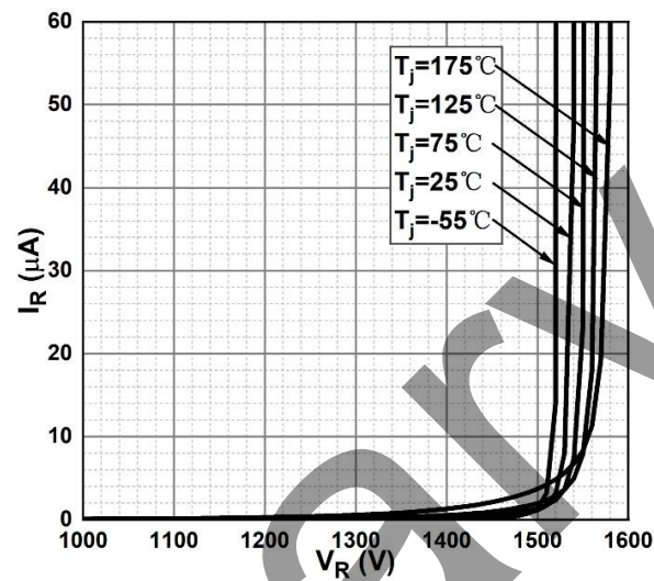
Figure 2. Reverse Characteristics
