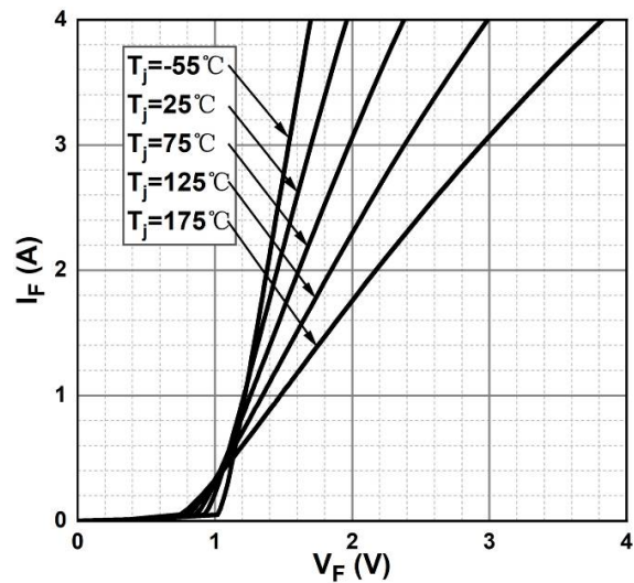
Figure 1. Forward Characteristics
