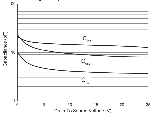
Fig. 5 - Capacitance Characteristics
