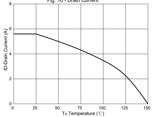
Fig. 10 - Drain Current
