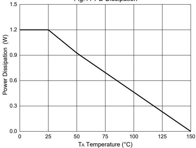
Fig.11-PD Dissipation
