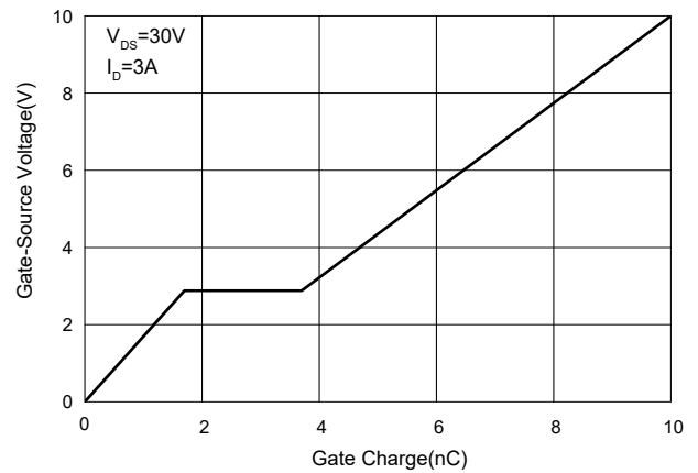
Fig. 6 - Gate Charge
