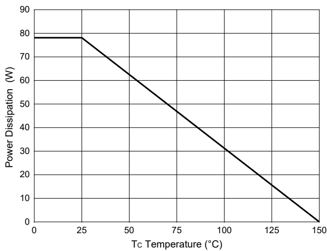
Fig.11-PD Dissipation
