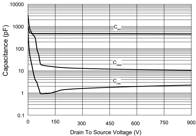
Fig.5 - Capacitance Characteristics
