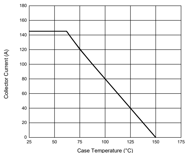
Fig. 11 - Collector Current vs. Case Temperature
