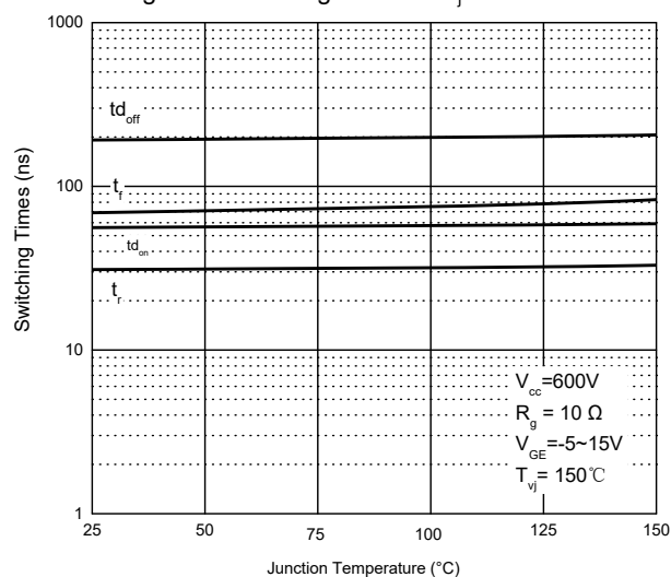
Fig. 13 - Switching Time vs. T_j
