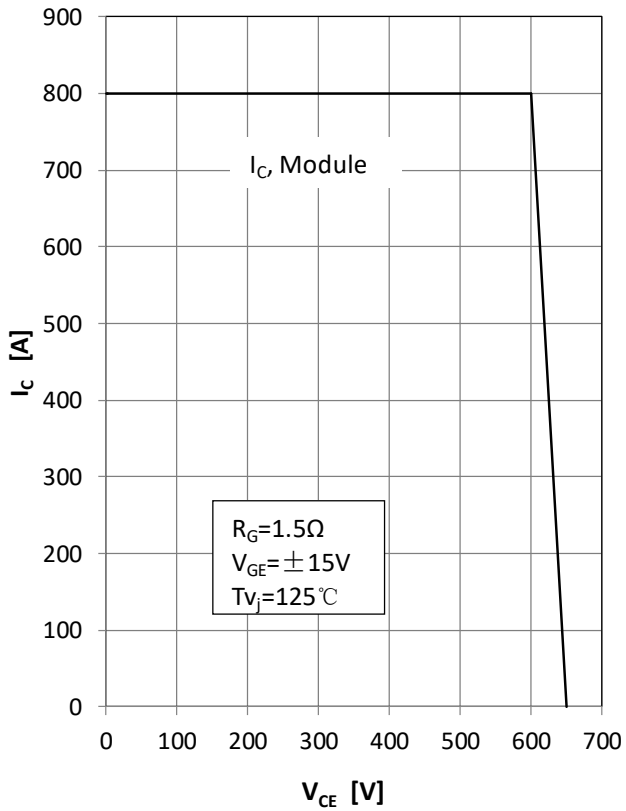
Fig5. RBSOA
