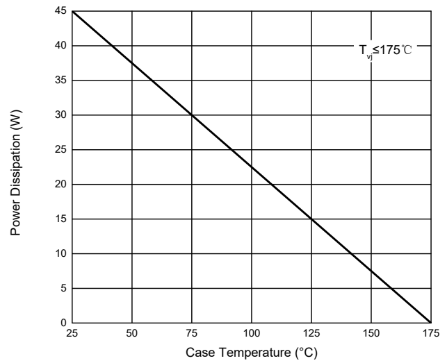
Fig. 16 - Power Derating
