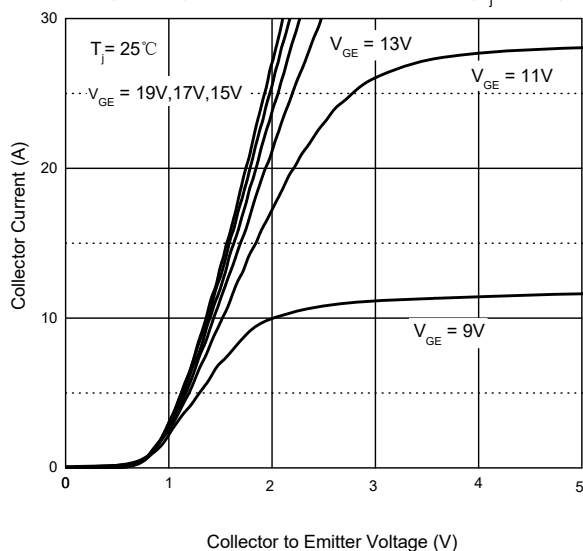
Fig. 1 - Typical Output Characteristic( T_j=25^\circ\text{C} )
