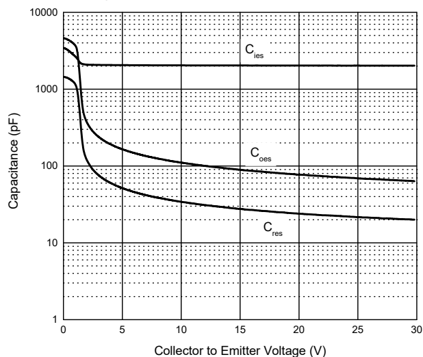
Fig. 5- Capacitance Characteristics
