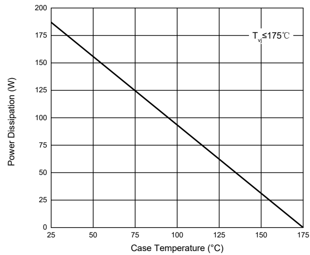
Fig. 14 - Power Derating
