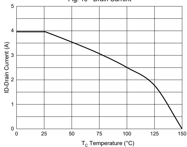
Fig. 10 - Drain Current
