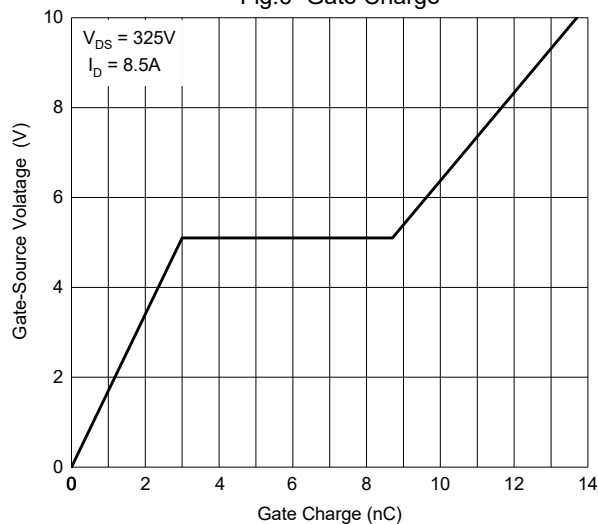
Fig.6- Gate Charge
