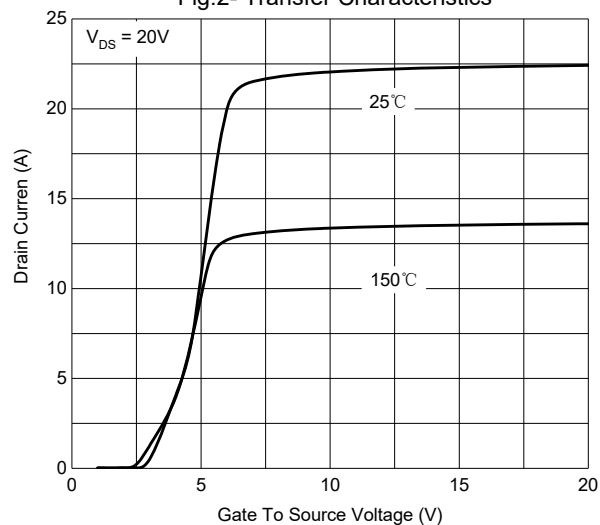
Fig.2- Transfer Characteristics
