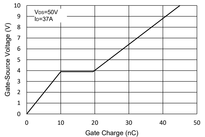
Fig.6 - Gate Charge
